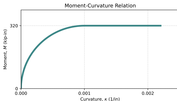
Fig. Adopted Moment Curvature Relationship
