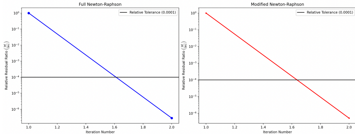
Part (b): Convergence comparison before yielding
