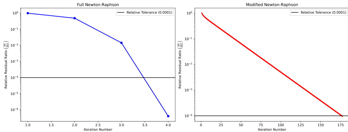
Part (b): Convergence comparison just after yield point
